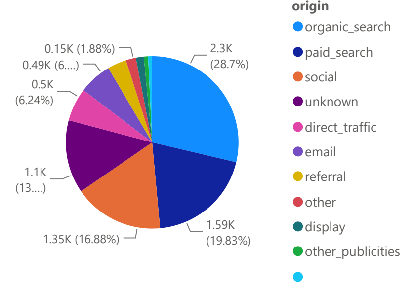
Count of mql_id by origin
