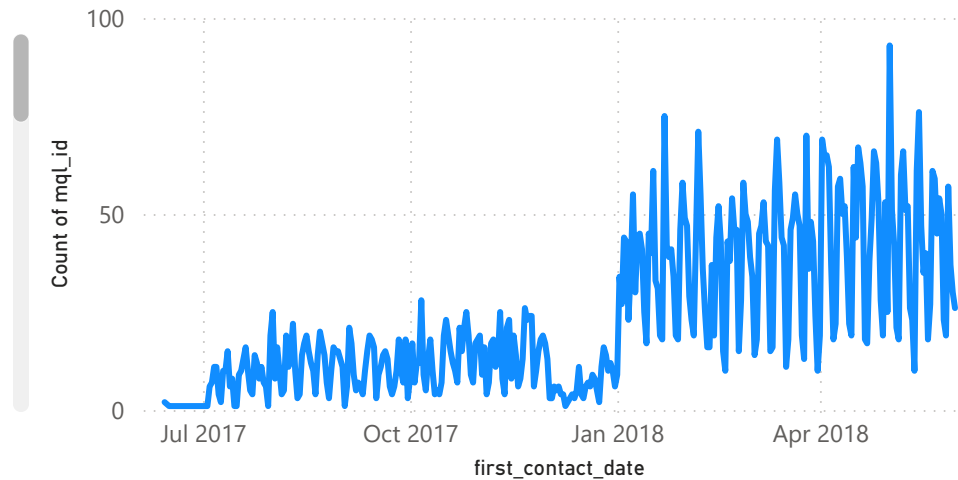
Count of mql_id by first_contact_date
