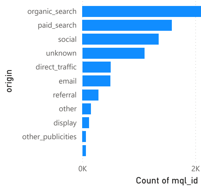
Count of mql_id by origin
