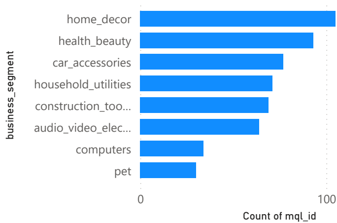
Count of mql_id by business_segment
